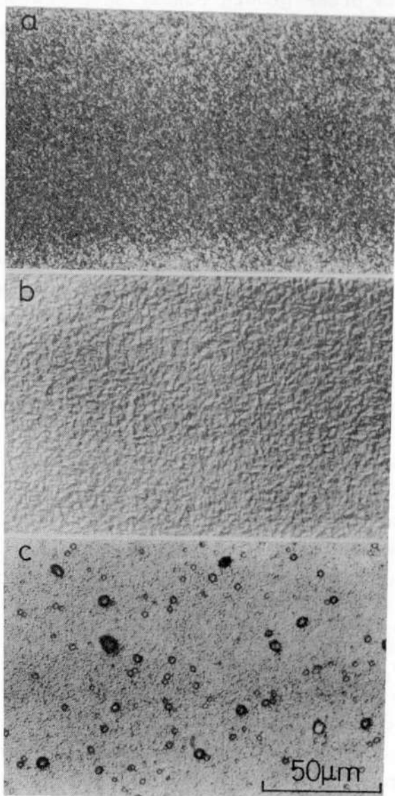
Fig.15 Si/C ratio dependence of surface morphology on Si(100). (a) Si-rich condition, Si/C=0.97, (b) moderate Si/C ratio, Si/C=0.34 and (c) C-rich condition, Si/C=0.27.
