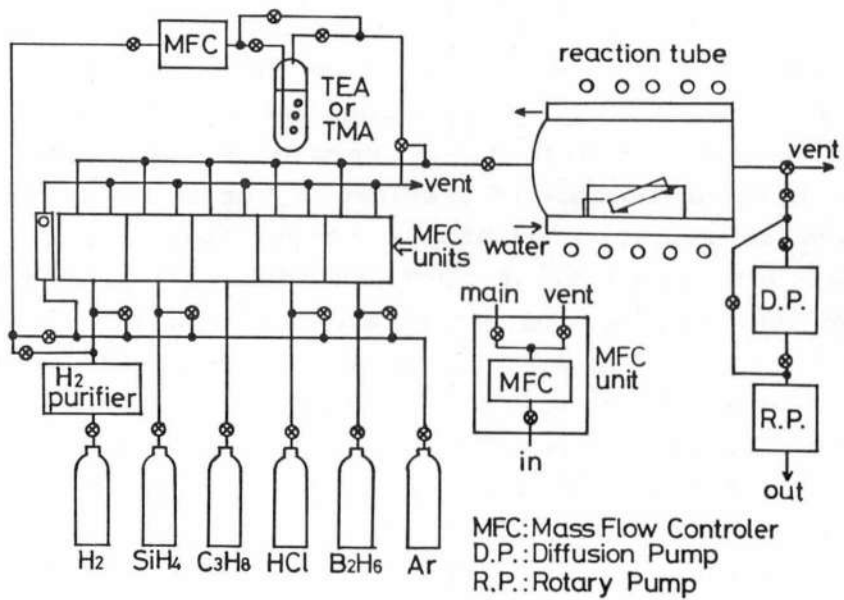
Fig.1 Schematic diagram of CVD growth system.
