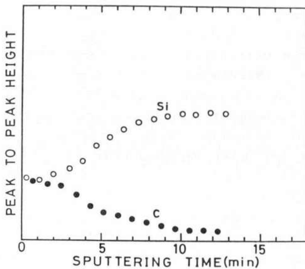
Fig.9 Auger electron spectroscopic depth profile of a carbonized buffer layer. An etching rate was about 3nm/min.
